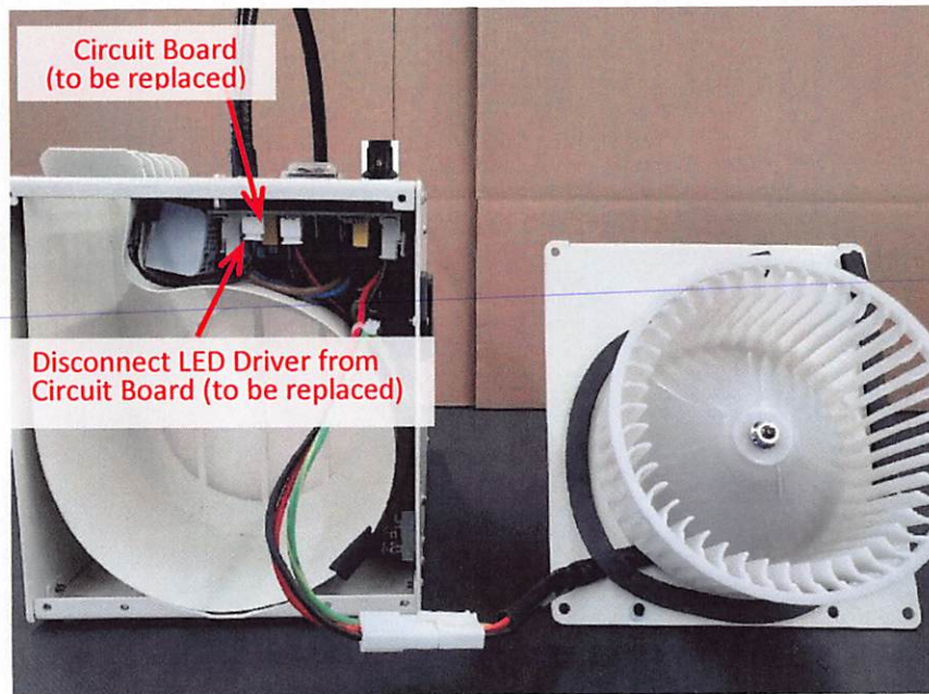
Figure 2. Shown with Rear Panel removed, and replaceable components identified.
